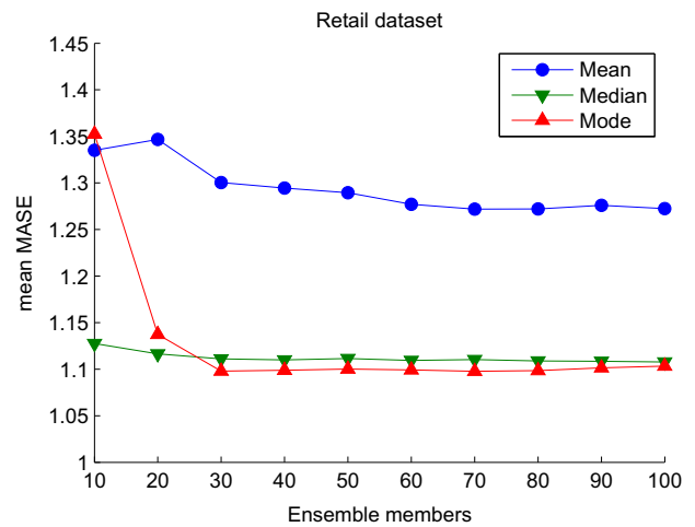
Fig. 5. Mean MASE for different number of ensemble members for the Retail dataset.
